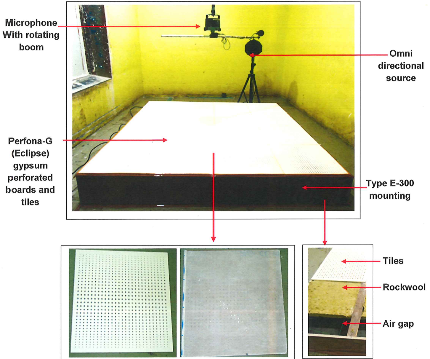
Figure 1: Test set up for mounting and testing of Perfona-G (Eclipse) gypsum perforated boards and tiles of 12 mm thick along with 300 mm air gap filled with 48 kg/m 3 density and 50 mm thick rockwool in reverberation chamber
