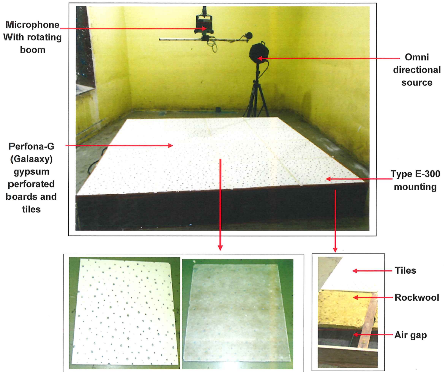
Figure 1: Test set up for mounting and testing of Perfona-G (Galaaxy) gypsum perforated boards and tiles of 12 mm thick along with 300 mm air gap filled with 48 kg/m 3 density and 50 mm thick rockwool in reverberation chamber
