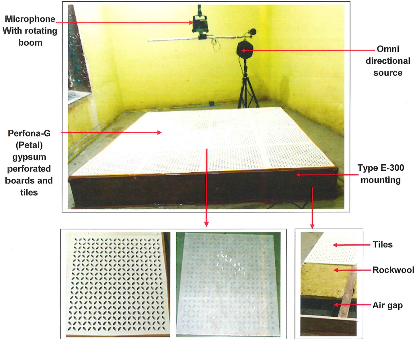
Figure 1: Test set up for mounting and testing of Perfona-G (Petal) gypsum perforated boards and tiles of 12 mm thick along with 300 mm air gap filled with 48 kg/m 3 density and 50 mm thick rockwool in reverberation chamber
