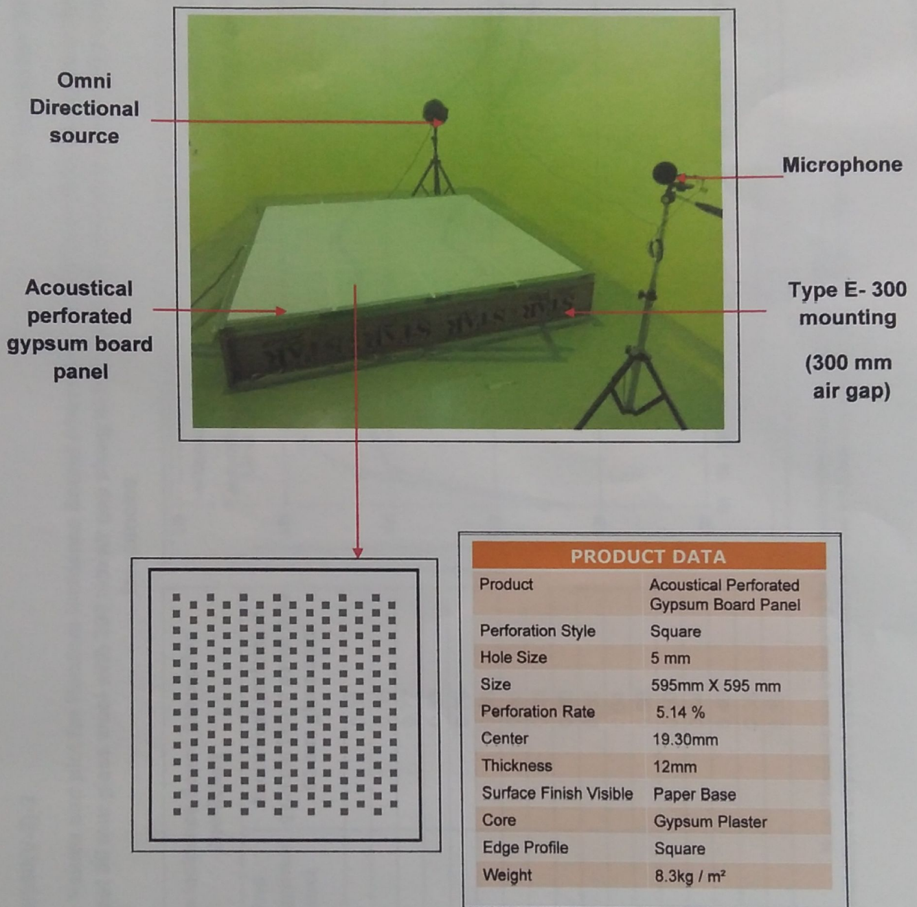
Figure 1: Test set up for mounting and testing of Acoustical perforated gypsum board panel in reverberation chamber
